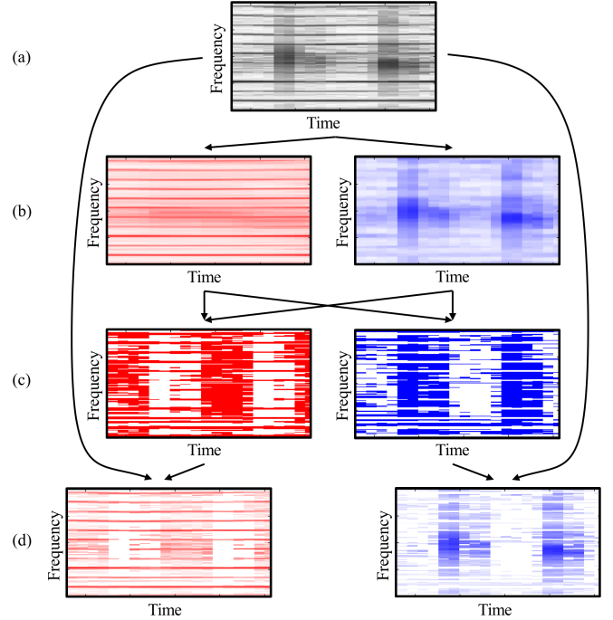
Fig. 2. Harmonic-percussive separation. (a): Spectrogram X . (b): Horizontally and vertically median-filtered magnitude spectrograms \tilde{Y}_h (left) and \tilde{Y}_p (right). (c): Binary masks M_h (left) and M_p (right) derived from \tilde{Y}_h and \tilde{Y}_p . (d): Masked spectrograms X_h (left) and X_p (right).
