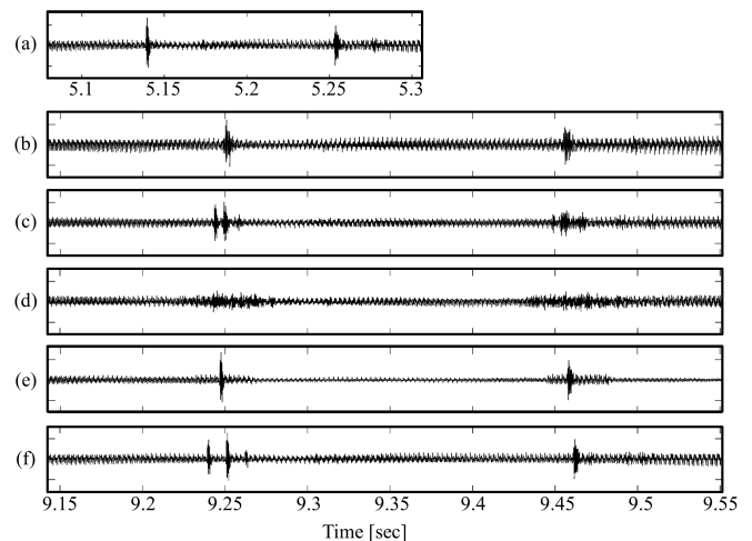
Fig. 3. (a): Excerpt of the CastanetsViolin Item. (b)-(f): TSM results for a constant stretching factor of 1.8 of (b): HP (c): EL (d): PV (e): NW (f): WS.
